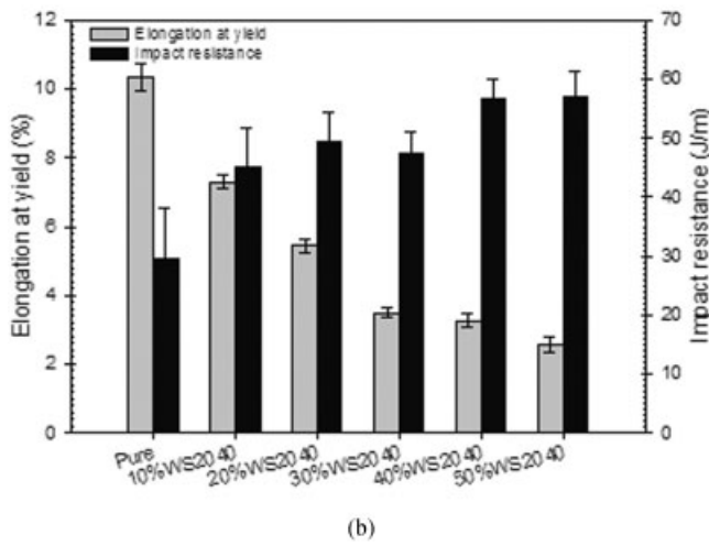
Figure 8 (a) Tensile strength at yield and Young's modulus and (b) elongation at yield and Izod impact resistance for pure and WS (20–40) fiber-reinforced iPP composites of varying fiber content (ranging from 10 to 50 wt %).
