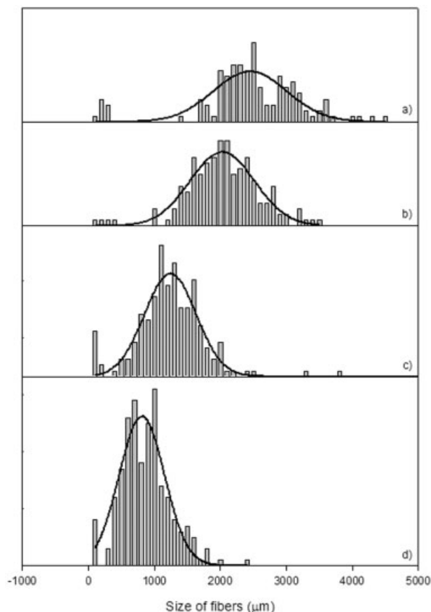
Figure 1 Lengths of as-prepared roselle (core, WS, or WC) fibers: (a) mesh >20, (b) mesh 20–30, (c) mesh 30–50, and (d) mesh <50.
