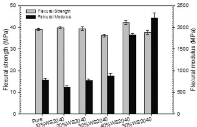
Figure 9 Flexural strength and flexural modulus for pure and WS (20–40) fiber-reinforced iPP composites of varying fiber content (ranging from 10 to 50 wt %).
