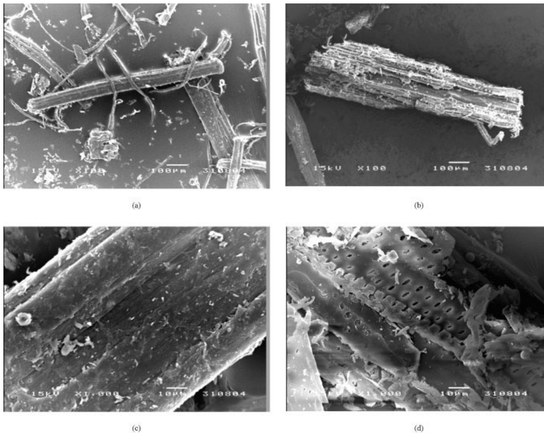
Figure 2 SEM images of (a) bast (×100), (b) core (×100), (c) bast (×1000), and (d) core fibers (×1000).
