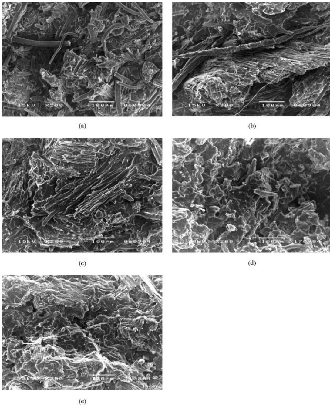
Figure 12 SEM images of surfaces of some impact specimens of 40 wt % WS (20–40) fiber-reinforced iPP composites compatibilized with (a) 1, (b) 3, (c) 5, (d) 7, and (e) 10 wt % MAPP.
