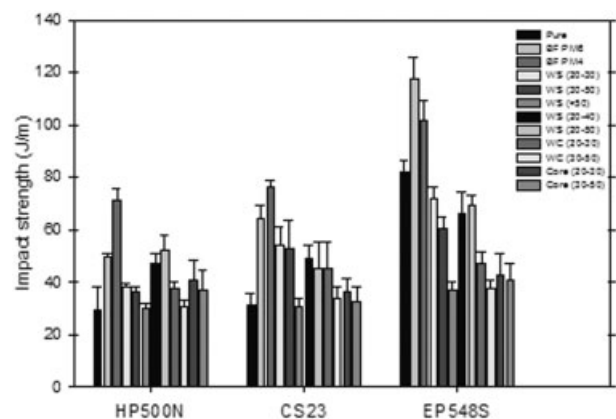
Figure 5 Izod impact resistance for all the as-prepared roselle fiber-reinforced iPP composite materials at a fixed fiber loading of 30 wt %.
