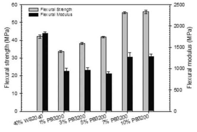
Figure 11 Flexural strength and flexural modulus for uncompatibilized and compatibilized 40 wt % WS (20–40) fiber-reinforced iPP composites of varying MAPP content (ranging from 1 to 10 wt %).
