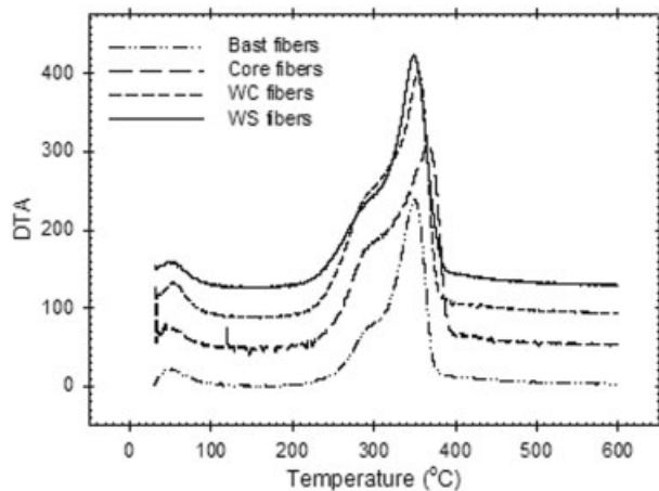
Figure 3 Derivative TGA spectra of roselle bast, WS, WC, and core fibers.
