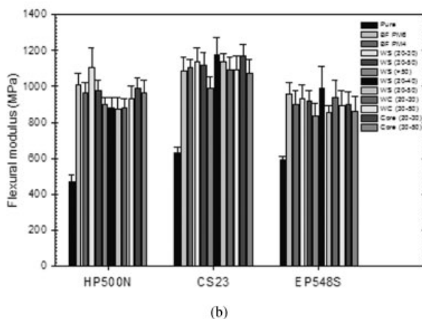
Figure 7 (a) Flexural strength and (b) flexural modulus for all the as-prepared roselle fiber-reinforced iPP composite materials at a fixed fiber loading of 30 wt %.
