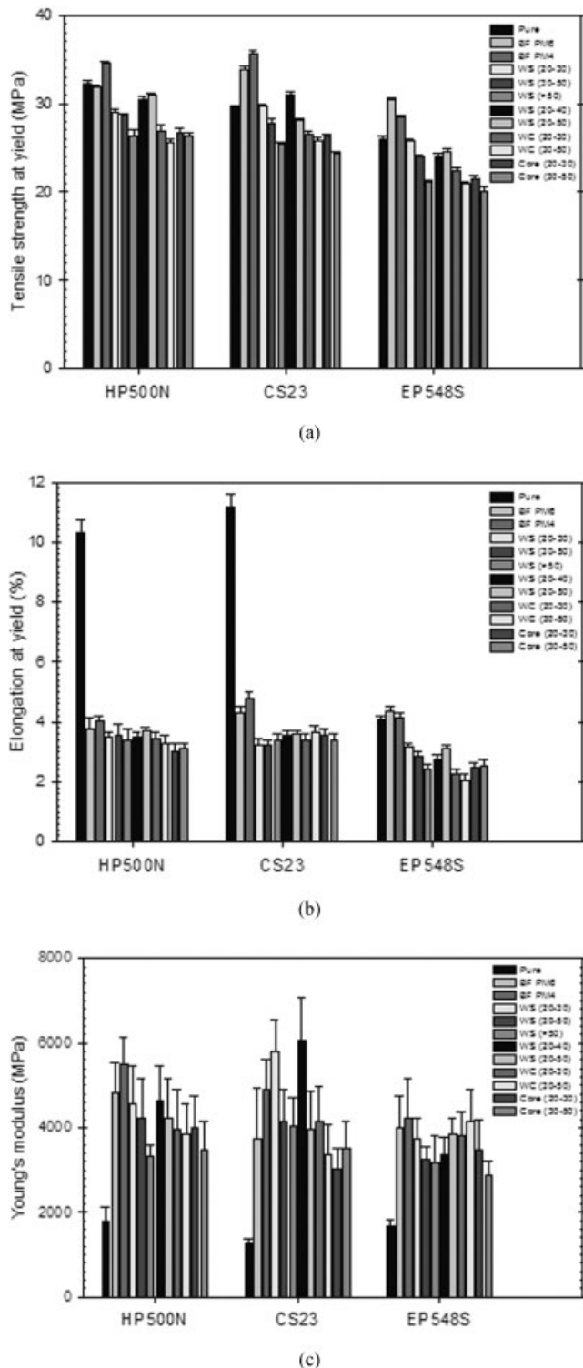
Figure 4 (a) Tensile strength at yield, (b) elongation at yield, and (c) Young's modulus for all the as-prepared roselle fiber-reinforced iPP composite materials at a fixed fiber loading of 30 wt %.
